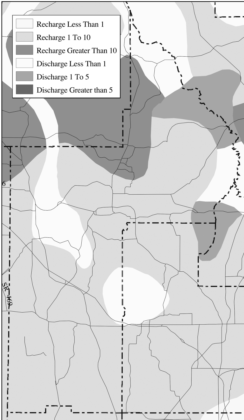
Withlacoochee River Watershed Recharge to/Discharge from the Floridan Aquifer In Inches Per Year- Lake County, May 9, 2001
