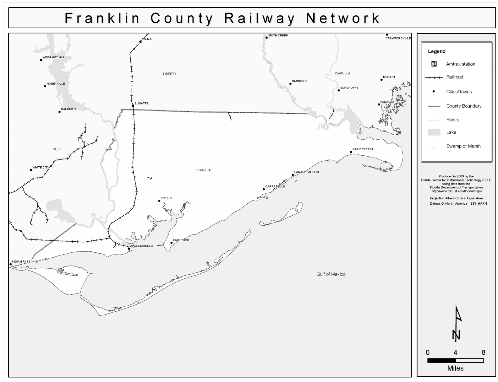
Franklin County Railway Network- Color, 2009
