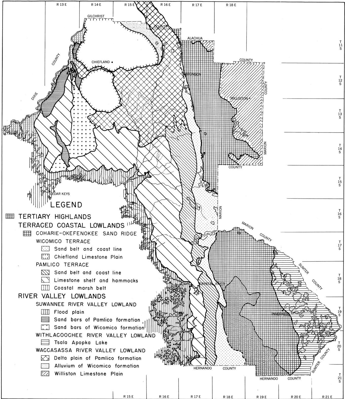
Physiographic map of Citrus and Levy counties, Florida.
