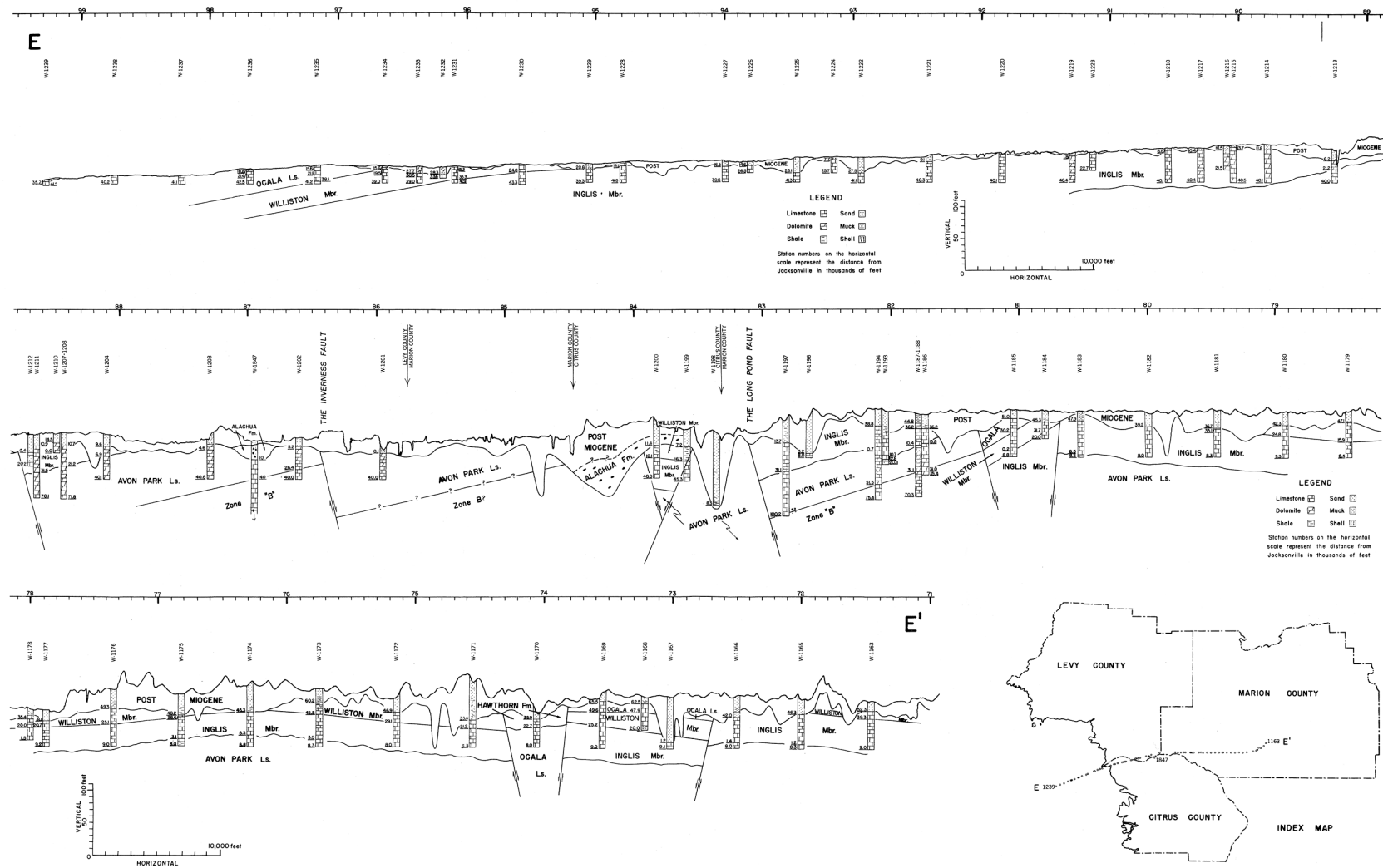
Geologic section along proposed route 13-B of the "Florida Ship Canal."
