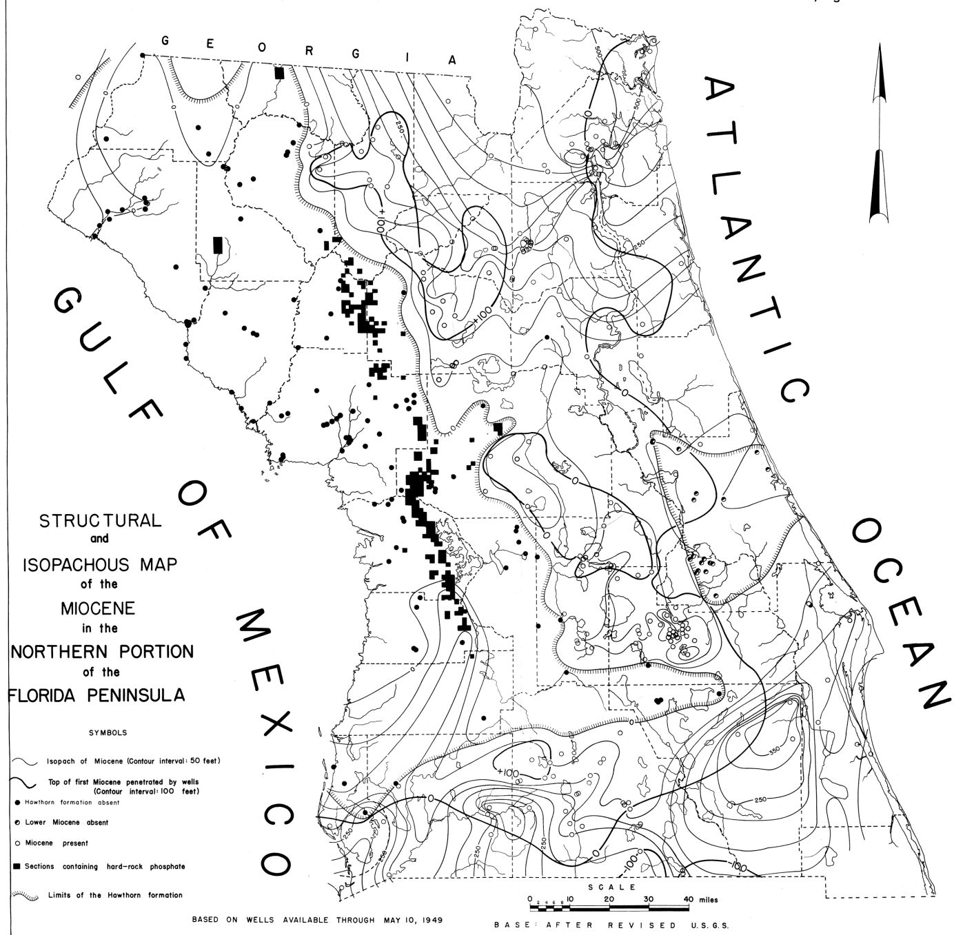
Miocene Structure and Isopach.
