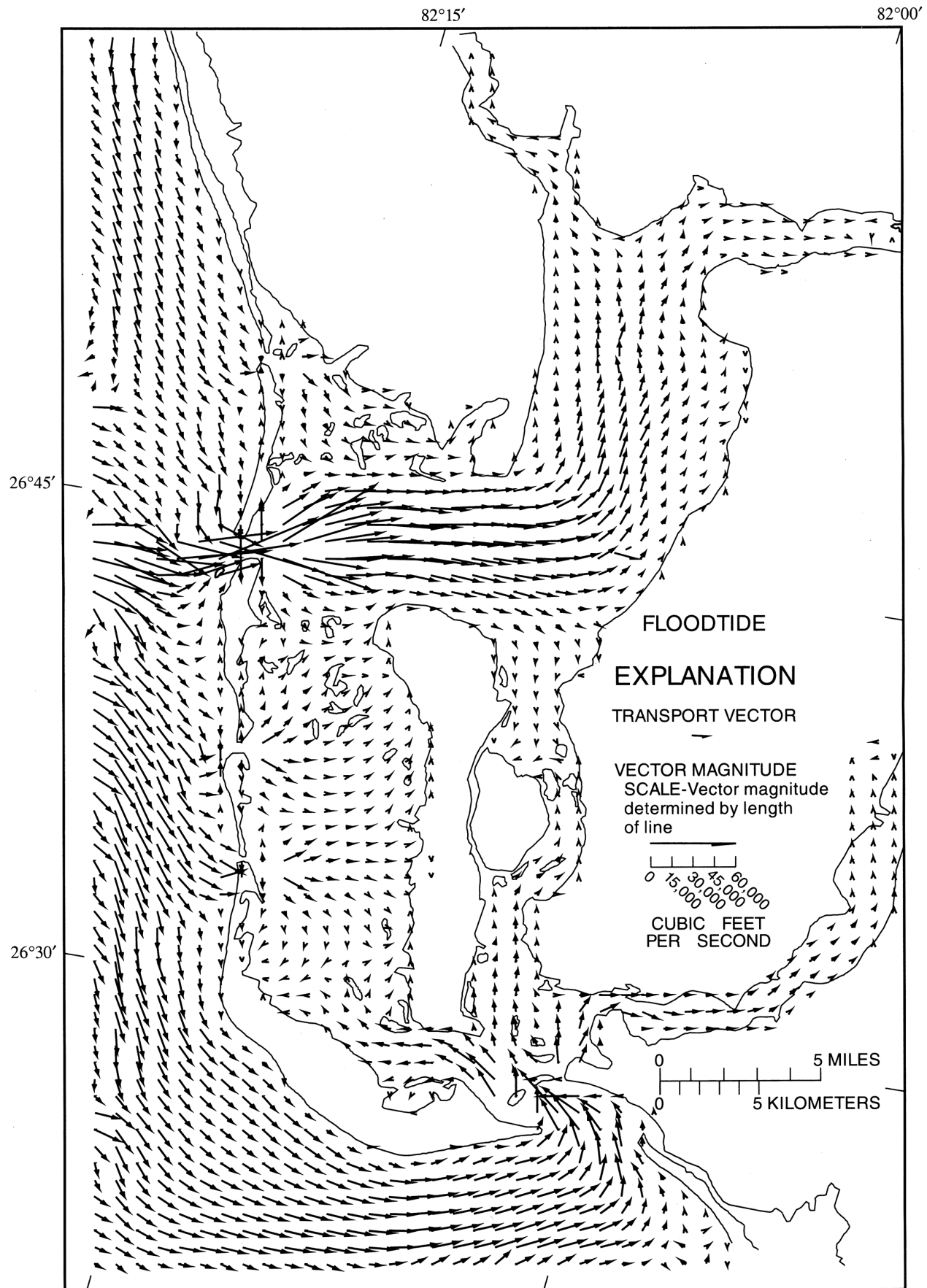
Floodtide Water Transport Vectors in Charlotte Harbor, 1996
