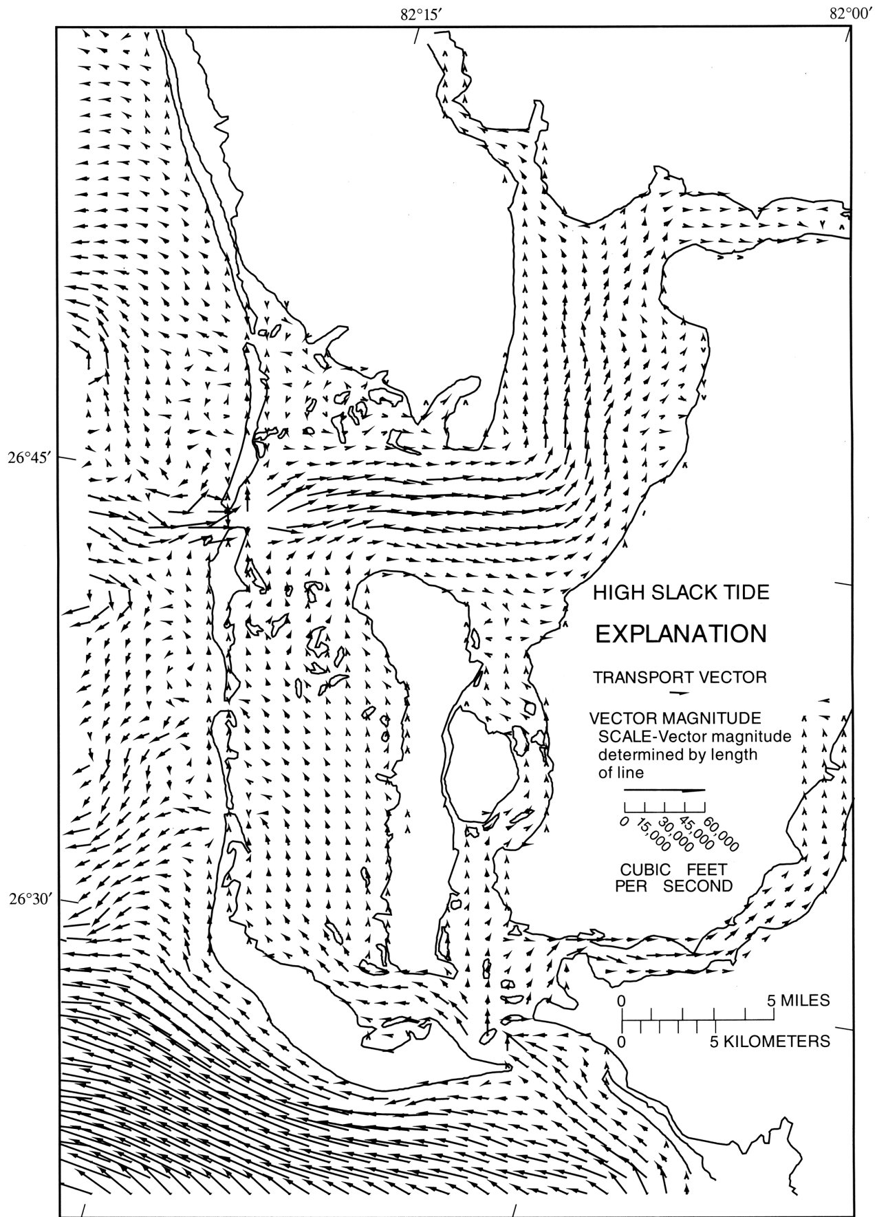
High Slack Tide Water Transport Vectors in Charlotte Harbor, 1996
