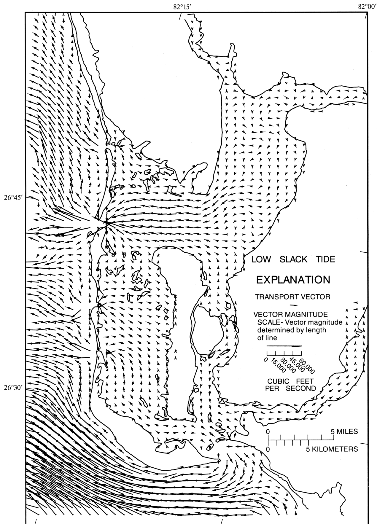
Low Slack Tide Water Transport Vectors in Charlotte Harbor, 1996
