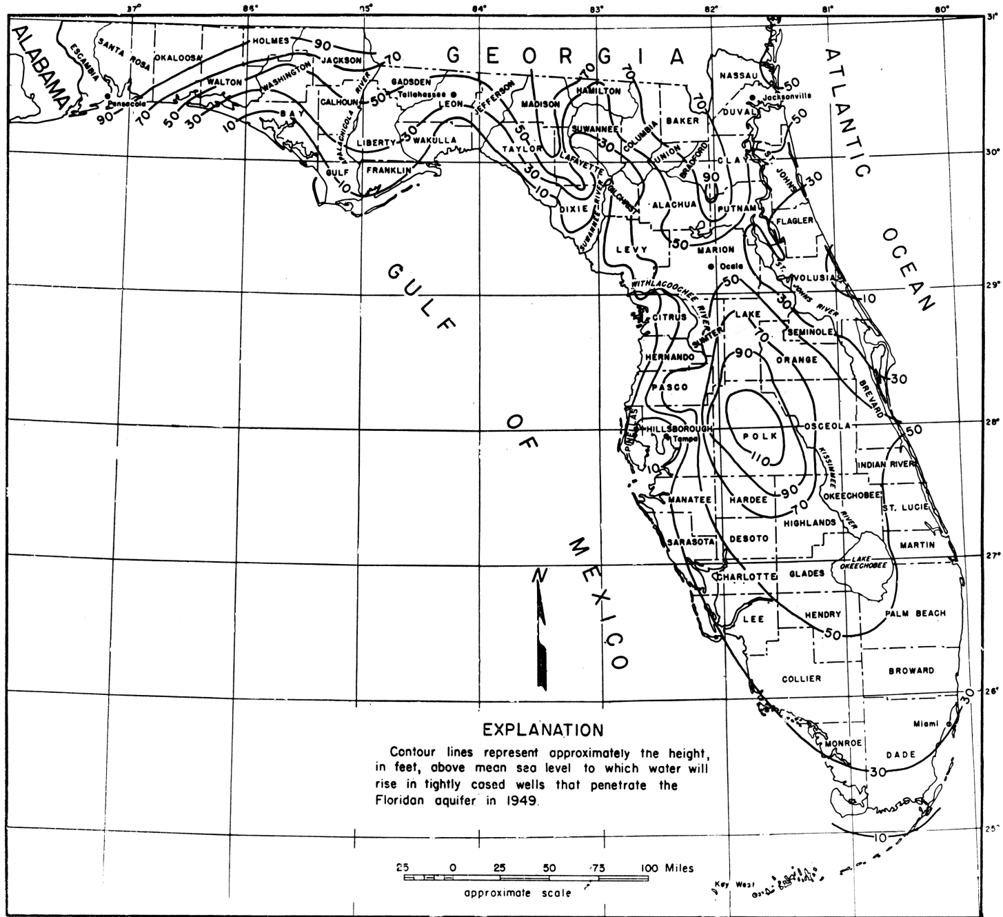
Piezometric Surface of the Floridian Aquifer, 1949
