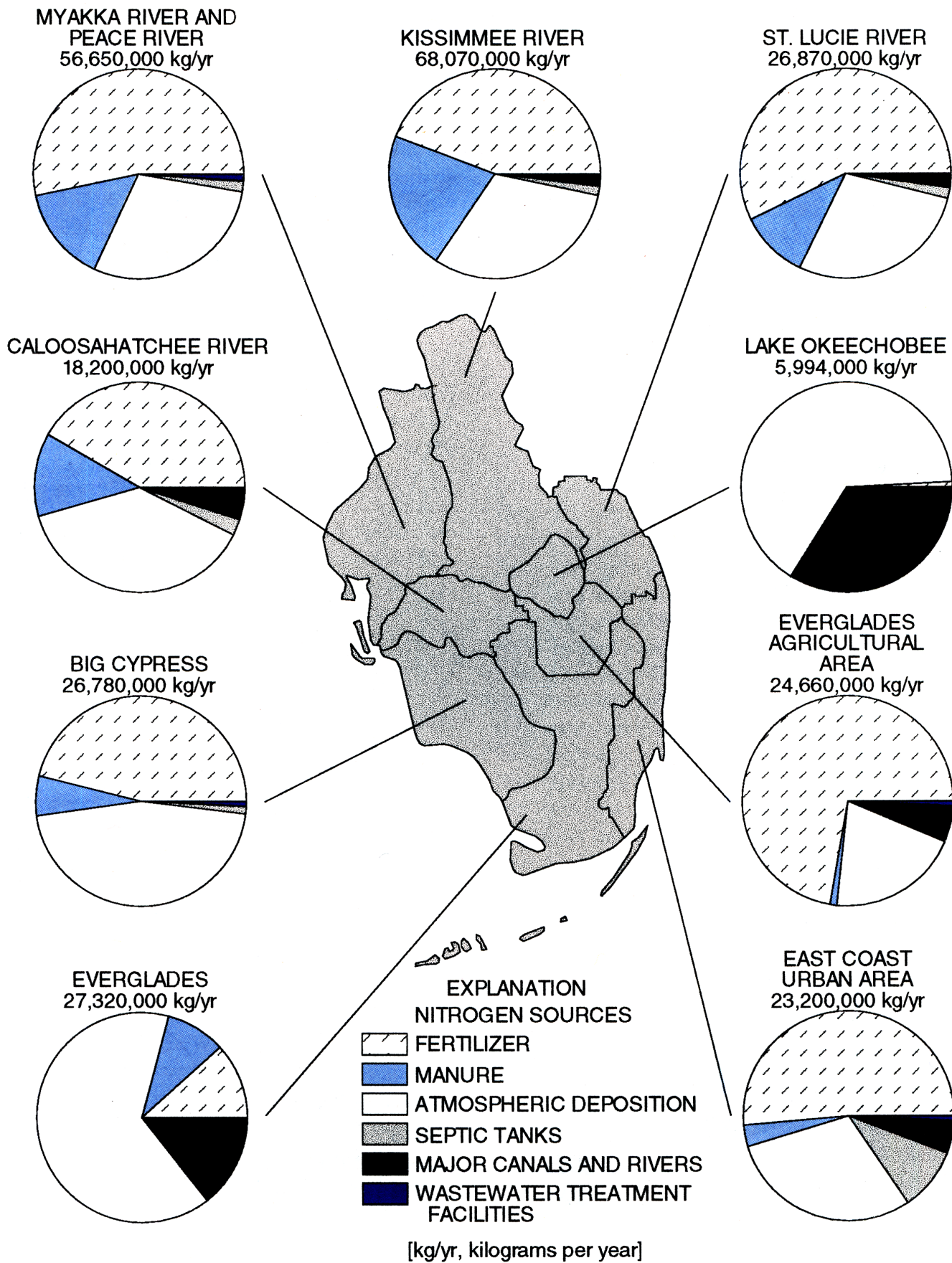
Nitrogen Loading in Surface Water Basins of Southern Florida, 1996
