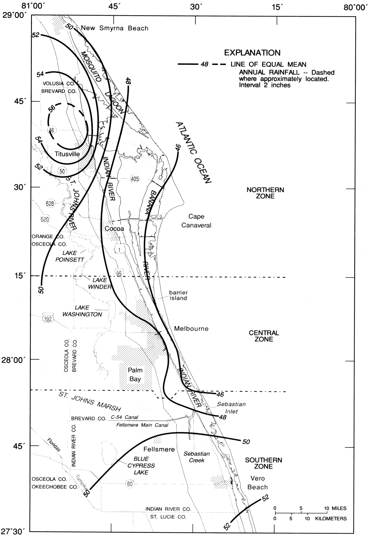
Mean Annual Rainfall in the Indian River Basin, 1951-1980
