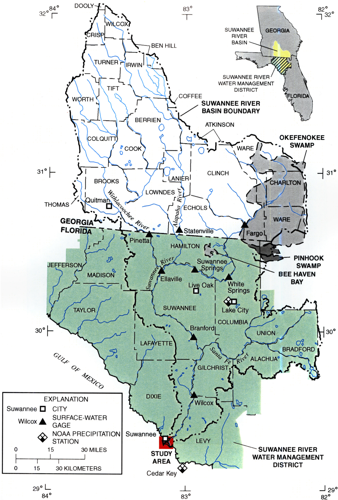
Suwannee River Basin Study Area Fig. 1, 2000
