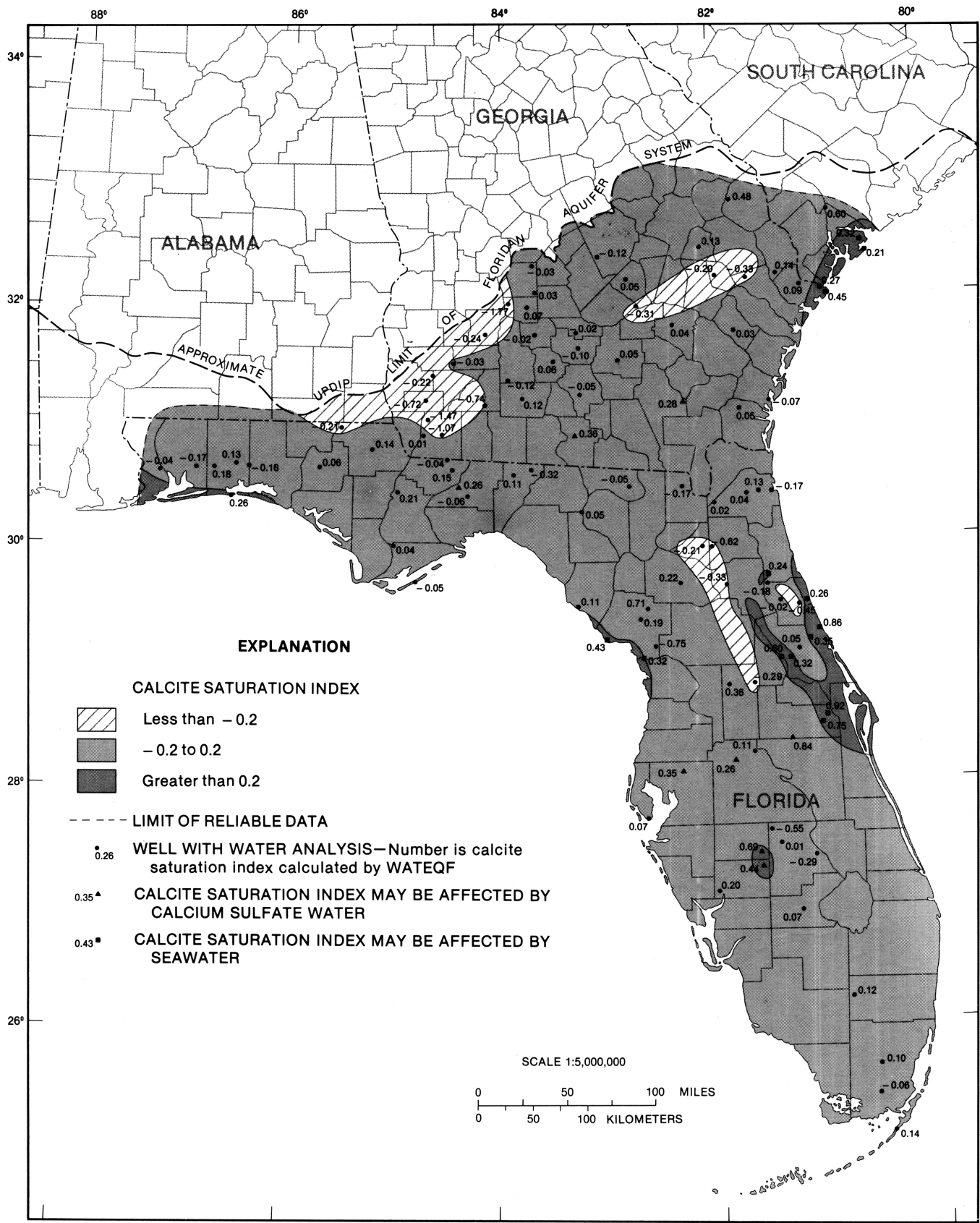
Calcite Saturation Index from the Upper Floridan Aquifer Fig 16, 1989
