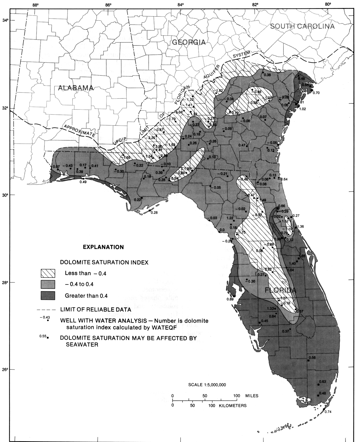
Dolomite Saturation Index from the Upper Floridan Aquifer Fig 18, 1989
