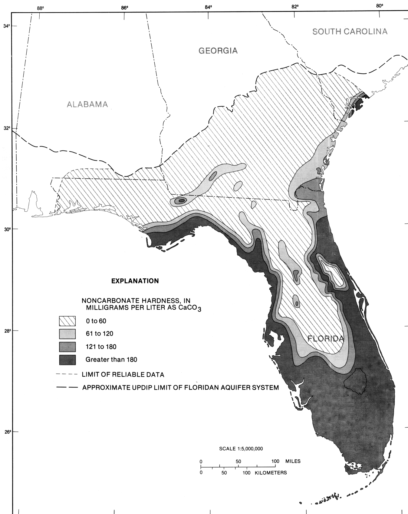
Noncarbonate Hardness of Water from the Upper Floridan Aquifer Fig 20, 1989 Craig L. Sprinkle, USGS Professional Paper 1403-1 (Washington, : U. S. Government Printing Office, 1989) 14 Downloaded from Maps ETC , on the web at http://etc.usf.edu/maps [map #f9133]
