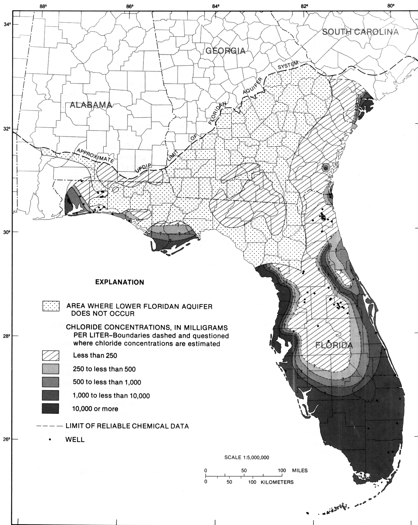
Chloride Concentrations from the Lower Floridan Aquifer Fig 24, 1989 Craig L. Sprinkle, USGS Professional Paper 1403-1 (Washington, : U. S. Government Printing Office, 1989) Downloaded from Maps ETC , on the web at http://etc.usf.edu/maps [map #f9140]
