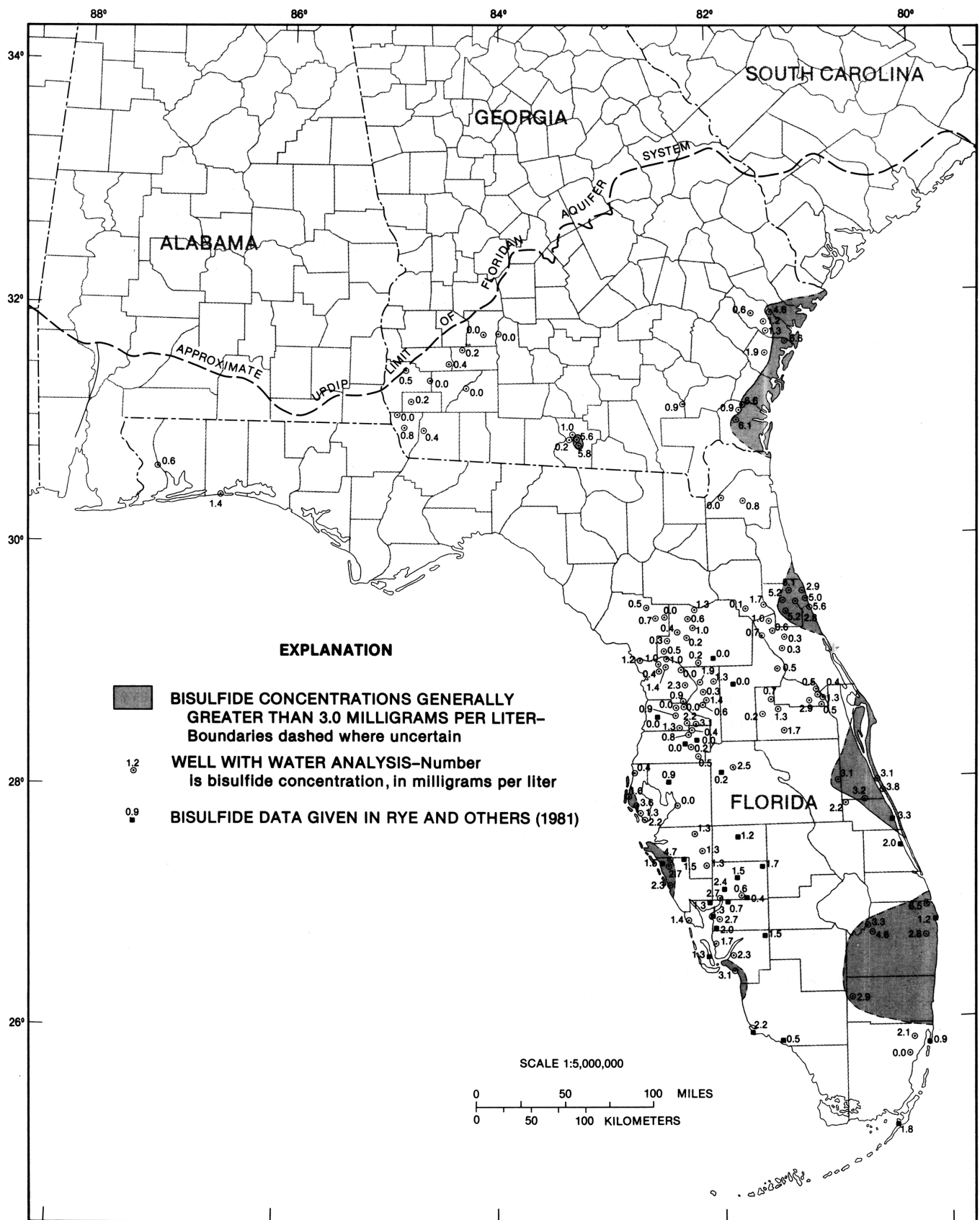
Bisulfide Concentrations in the Upper Floridan Aquifer Fig 26, 1989
