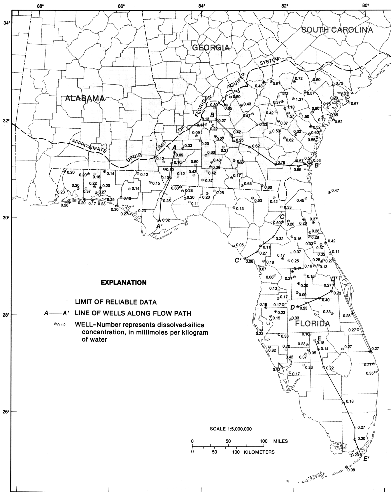
Concentrations of Dissolved Silica from the Upper Floridan Aquifer Fig 30, 1989 Craig L. Sprinkle, USGS Professional Paper 1403-1 (Washington, : U. S. Government Printing Office, 1989) Downloaded from Maps ETC , on the web at http://etc.usf.edu/maps [map #f9144]
