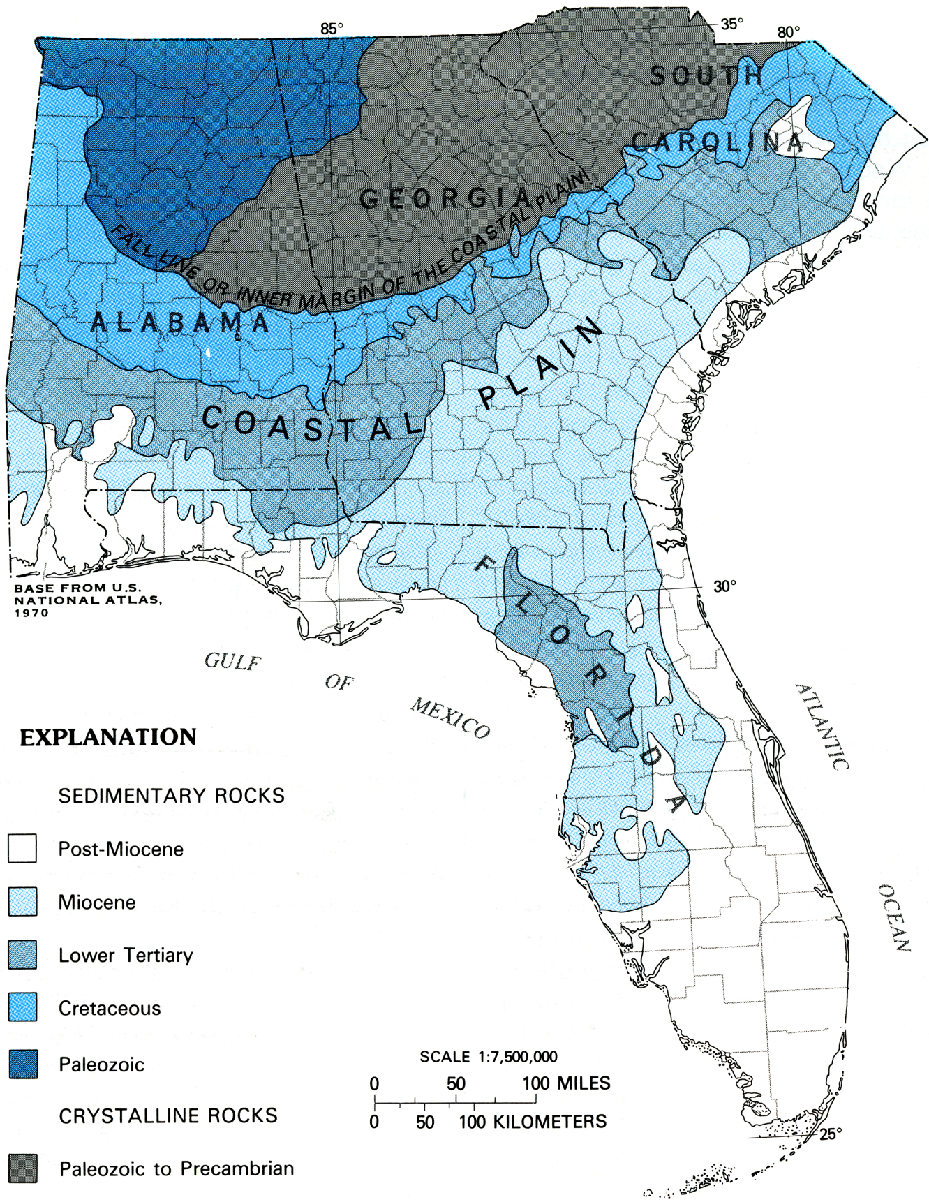
Generalized Geologic Map of the Southeastern United States, 1988 P. W. Bush and R. H. Johnston, USGS Professional Paper 1403-C (Washington, DC: U. S. Government Printing Office, 1988) C4
