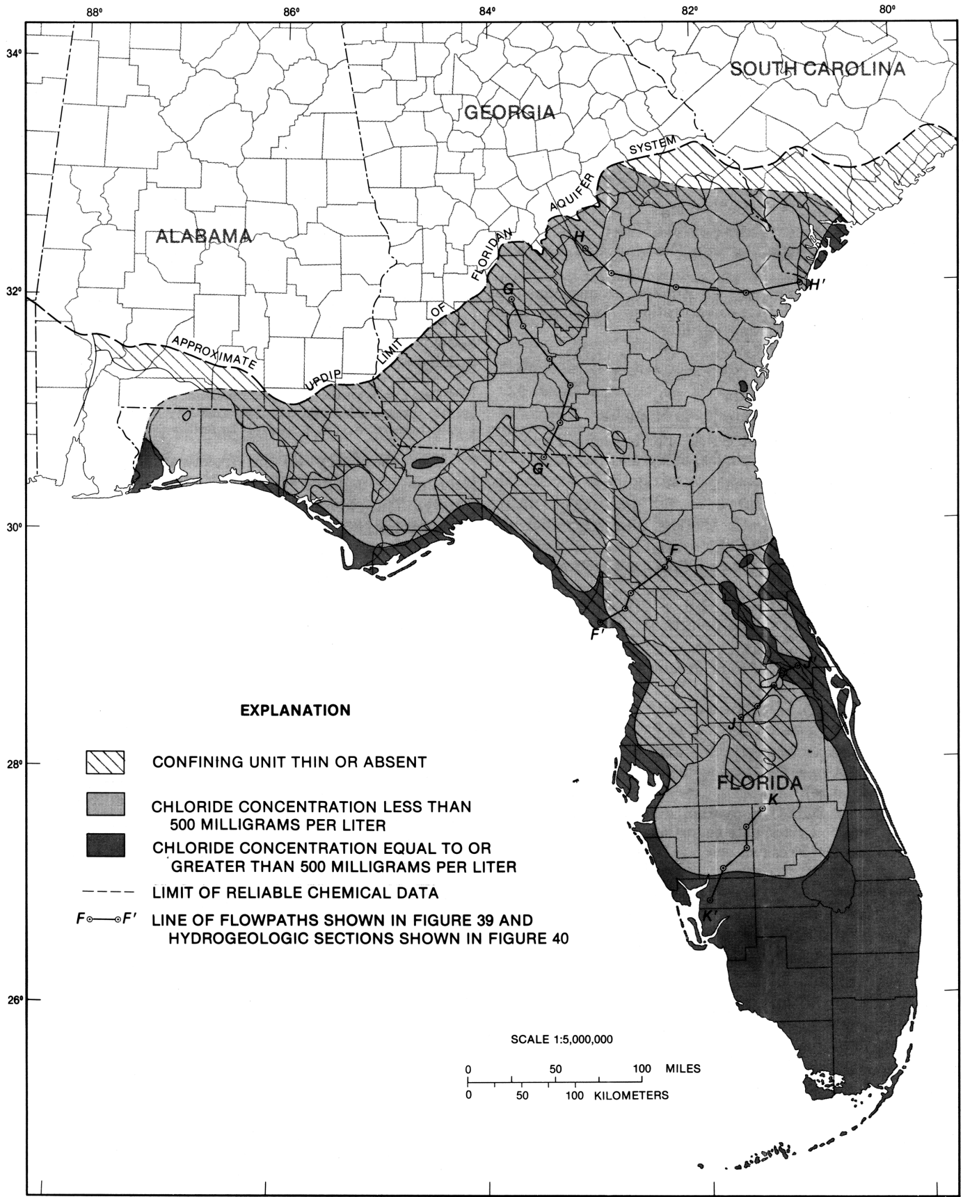
Relation of Chloride Concentrations to Confined-Unconfined Conditions Fig 38, 1989 Craig L. Sprinkle, USGS Professional Paper 1403-1 (Washington, : U. S. Government Printing Office, 1989) 185 Downloaded from Maps ETC , on the web at http://etc.usf.edu/maps [map #f9222]
