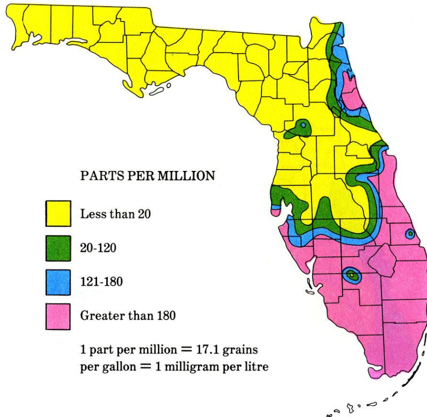
NON-CARBONATE HARDNESS OF WATER FROM THE FLORIDAN AQUIFER IN FLORIDA.
