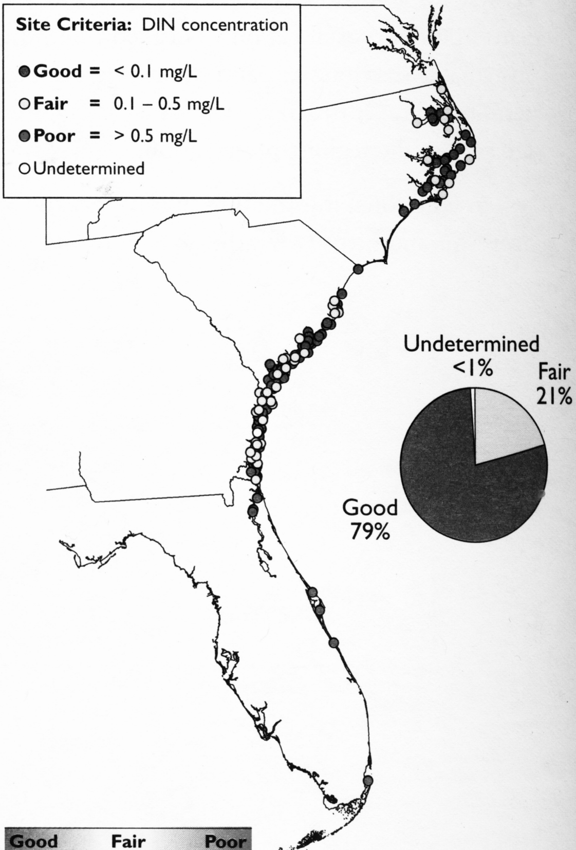
Nitrogen in Southeast, 2000
