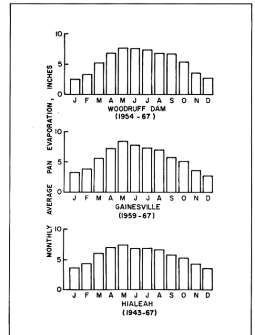
Figure 2. Monthly Average Pan Evaporation at Woodruff Dam, Gainesville, and Hialeah.
